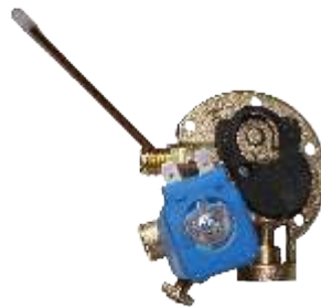
9.02.5000.900030 30° CYLINDER MULTIVALVE
