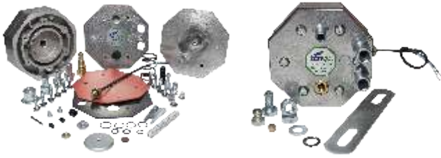
0.02.0301.000001 SEQUENTIAL REDUCER
